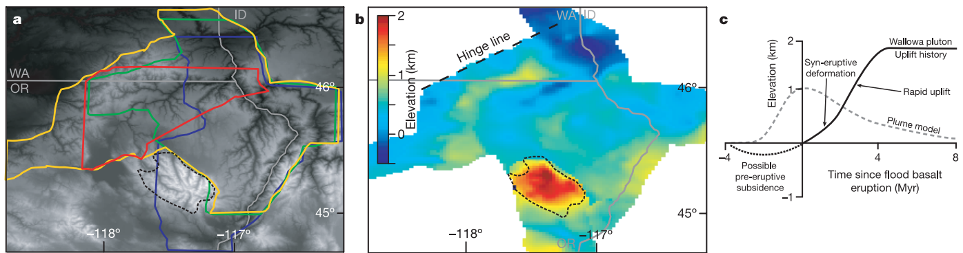
Figure 2 | Maps of post-eruptive uplift in the Wallowa Mountains area. a , Digital elevation map showing the overlapping distribution of exposed Grande Ronde magmatographic interfaces used for analysis of Wallowa Mountains uplift: Imnaha-R1 (blue), R1-N1 (green), N1-R2 (yellow) and R2-N2 (red). b , Composite surface for Grande Ronde uplift. This surface was made by vertically shifting the individual interfaces using published flow thicknesses 14 , smoothing the resulting surface with a mild low-pass filter, and removing the effects of erosional unloading by deconvolving the point load response of an elastic plate 17,18 , assuming total coverage by the Grande Ronde lavas and an elastic thickness of 5 km, similar to other estimates from this area 22 . The absolute elevation is referenced to a hinge line (dotted black line) that separates the uplifted Blue Mountains from the down-dropped Pasco basin immediately northwest of the Blue Mountains. c , Schematic plot
