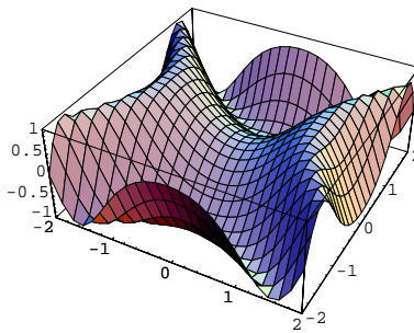
Figure 1: from Mathematica
