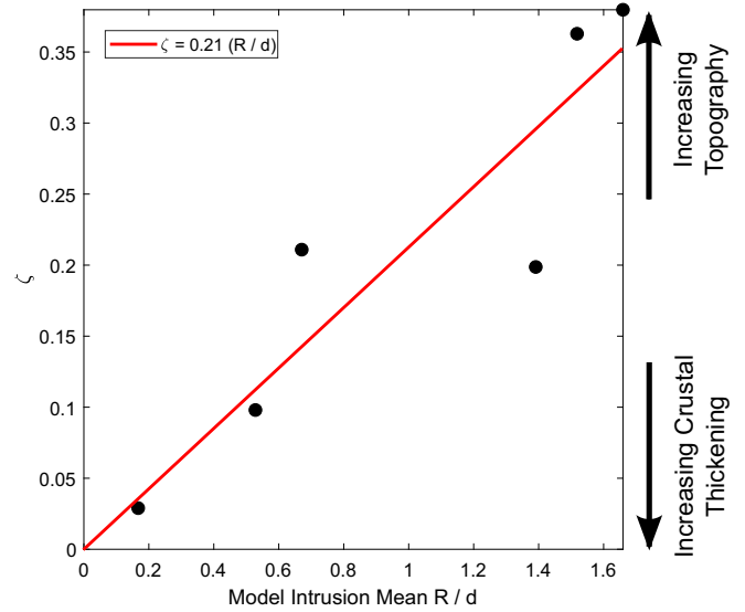
Fig. 5. Volume of topographic relief divided by volume of crustal thickening associated with stochastic intrusions ( \zeta ; Eq. (5)), ordered by mean model intrusion radius-to-depth ratio for Poisson spatial intrusion distributions. Red line is best-fitting linear fit of data.
