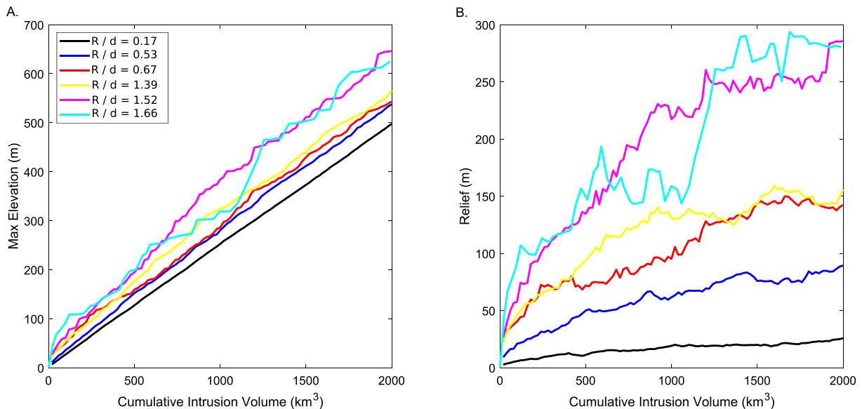
Fig. 4. (A) Maximum elevation and (B) relief of model topography as a function of cumulative intrusive volume for Poisson spatial intrusion distribution models, illustrating our stochastic simulation procedure. Colors correspond to model parameters presented in legend, showing increasing topography with increasing R/d .
