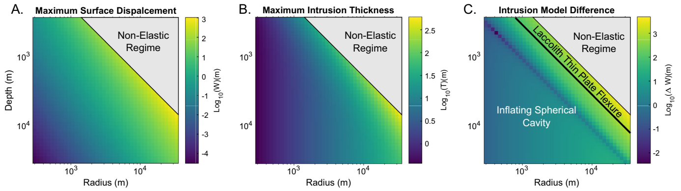
Fig. 1. Stochastic model intrusion radius-depth ( R - d ) parameter space using the pressurized penny-shaped crack displacement model (Fialko et al., 2001). A: Maximum surface displacement. B: Maximum intrusion thickness. C: Displacement difference between pressurized penny-shaped crack and typical inflating point source (McTigue, 1987) and thin-plate flexure (Galland and Scheibert, 2013) models. Black line represents parameter values that create equal maximum surface displacements between inflating spherical cavity and thin-plate flexure models. Non-elastic regime defines the R/d limitation of the inflating penny-shaped crack model ( \sim 5.6 ; Fialko et al., 2001).
