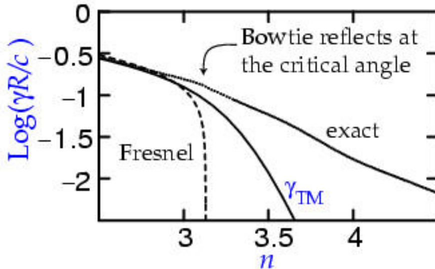
Figure 2: Width of a TM bowtie mode vs. refractive index, from numerical and ray calculations.
