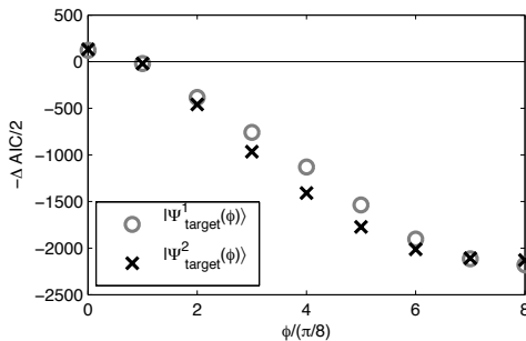
FIG. 2: Comparing single- and double-excitation Dicke states: The difference between AICs of M_{1\phi} and the FPM, i.e., -\Delta AIC = AIC(\text{FPM}) - AIC(M_{1\phi}) for both target states, when N = 10000 , as functions of \phi . The horizontal line demarcates \Delta AIC = 0 .
